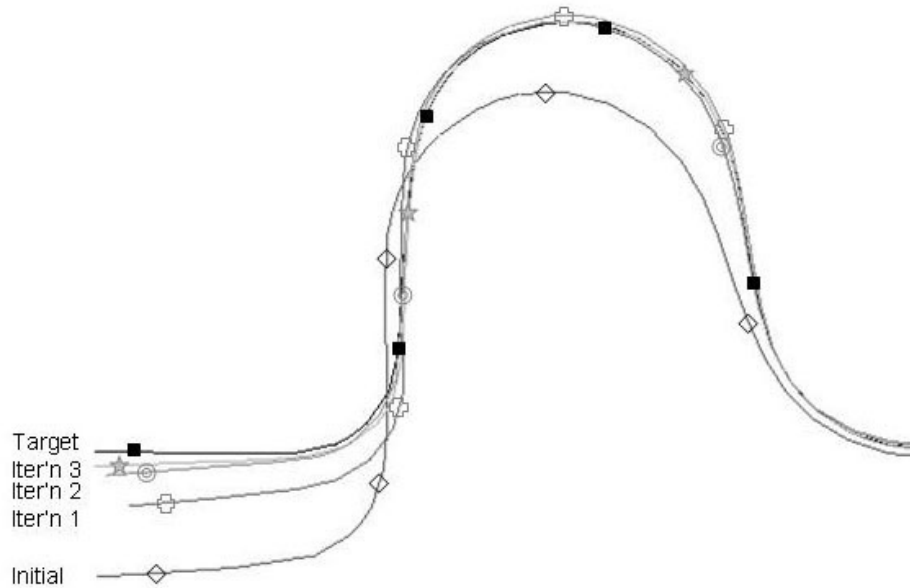
Figure 5: Results of Automated Springback Compensation; sections show trend from initial springback (diamonds) through three iterations (1=crosses, 2=circles and 3=stars), compared with the target geometry (squares)
